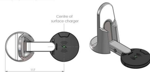
Charging configuration
